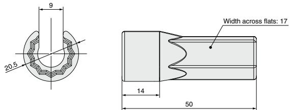
VCC-G-D-2 (Applicable fitting VCK \begin{smallmatrix} 0806 \\ 0604 \end{smallmatrix} )
