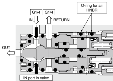
3 port valve
