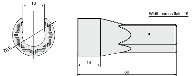
VCC-G-D-1 (Applicable fitting VCK \begin{smallmatrix} 1209 \\ 1008 \\ 1075 \end{smallmatrix} )
