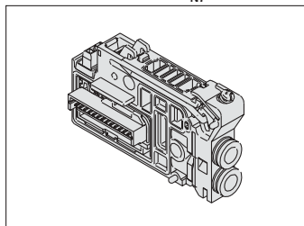
排气塞板组件 VVQC1000-19A-S D C3, C4, C6, M5, N1, N3, N7
